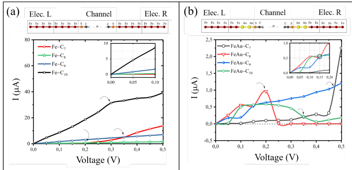
Fig.1. Coupled nanowires with carbon variation of 7 to 10 atoms. In (a) nanowire based solely on the bonding of Fe atoms with carbons and on (b) Fe-nanowire with Au interface attached to the carbon atoms.
